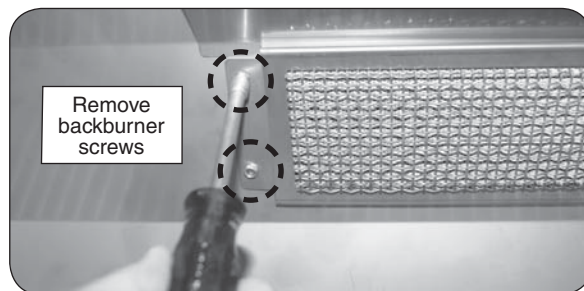
Fig. 29-5 Remove backburner mounting screws
